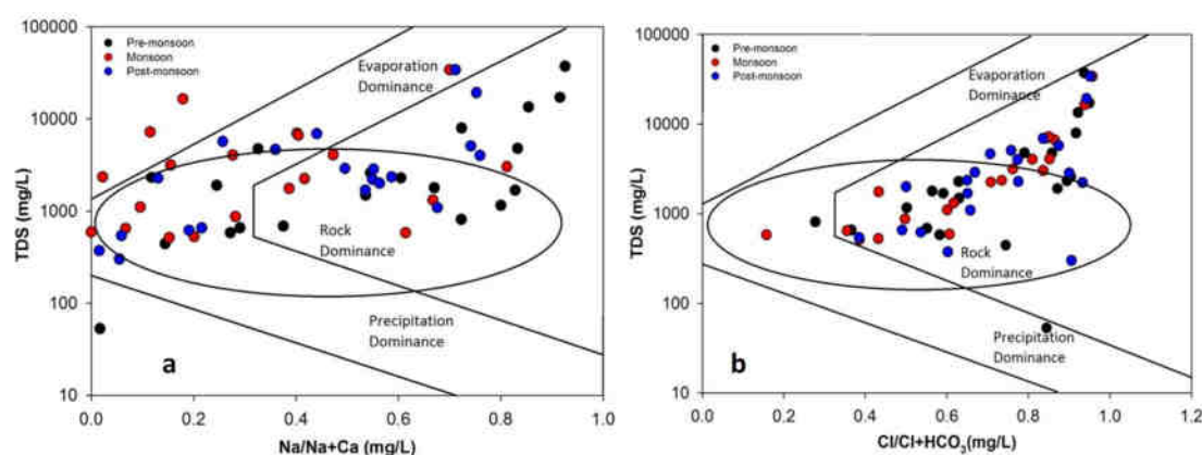
Figure 10. Gibbs plots (a) TDS v/s \text{Na}^+/\text{Na}^+ + \text{Ca}^{2+} and (b) TDS v/s \text{Cl}^-/\text{Cl}^- + \text{HCO}_3^- .
